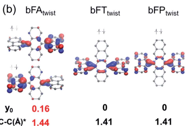
Fig. 5 (a) Energy diagram of bFA with rotation of the fluorene moiety; (b) HOMOs of the fluorene twisted structure of bFA ( \text{bFA}_{\text{twist}} ), bFT ( \text{bFT}_{\text{twist}} ), and bFP ( \text{bFP}_{\text{twist}} ), with the y_0 value and bond length (*) of the C–C bond between fluorene and acenes.
