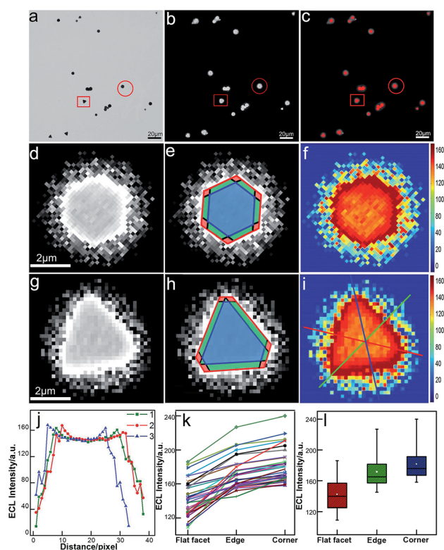
Fig. 2 Spatial distribution of ECL intensity on single gold nanoparticles. (a) Bright-field image, (b) ECL image (exposure time: 200 ms) and (c) false-color overlay of the bright-field and ECL images. (d and g) Magnified areas of the ECL image (b) marked by a red circle and square. (e and h) Divided regions of corners (red), edges (green), and the flat surface facet (blue) in the ECL images of (e and h). (f and i) 2D spatial distribution ECL intensity obtained by using Matlab. (j) ECL intensity gradients at three measuring lines marked in (i). (k) Statistical site-specific ECL intensity of 35 nanoparticles. (l) Box charts of the ECL intensities from corner, edge and flat facet regions.
