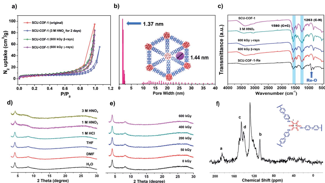
Fig. 2 (a) \text{N}_2 sorption isotherms of SCU-COF-1 after different treatments with 3 M \text{HNO}_3 , 600 kGy \beta -rays and 600 kGy \gamma -rays at 77 \text{ K} . (b) Pore size distribution of SCU-COF-1 calculated by NLDFT modelling based on \text{N}_2 adsorption data. (c) IR spectra of SCU-COF-1 and SCU-COF-1 after treatment with 3 M \text{HNO}_3 , 600 kGy \gamma -irradiation, 600 kGy \beta -irradiation, and stock solution containing \text{ReO}_4^- . (d) PXRD patterns of SCU-COF-1 after treatments in various solvents and acids for 48 h. (e) PXRD patterns of SCU-COF-1 after being irradiated with various doses of \beta -irradiation (50 kGy, 200 kGy, 400 kGy, 600 kGy). (f) ^{13}\text{C} solid NMR spectrum of SCU-COF-1.
