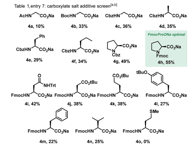
Scheme 2 Evaluation of amino acid additives. a Reaction conditions: 1a (0.05 mmol), 2a (0.1 mmol), [Cp*Rh(MeCN) 3 ](SbF 6 ) 2 (10 mol%), Fmoc-Pro-ONa (40 mol%), solvent (0.5 mL), temperature, 36 h. b Yield calculated by 1 H NMR with methyl para -nitrobenzoate as internal standard.
