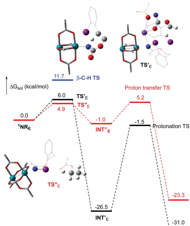
Fig. 12 Calculated free energy profile for the reactivity of \text{NR}_\text{E} at the PBE/BS2 level of theory (the relative free energies ( \Delta G_{\text{sol}} , kcal mol ^{-1} ) in ethyl acetate are provided). (Different atom styles are used for clarity.)
