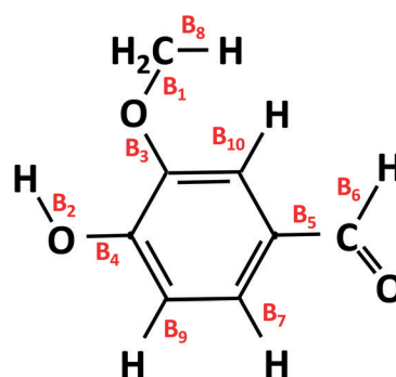
Vanillin
