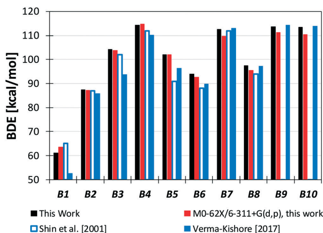
Fig. 3 BDEs of vanillin [kcal mol −1 ]. Comparison of literature 48,50 and predicted values.
