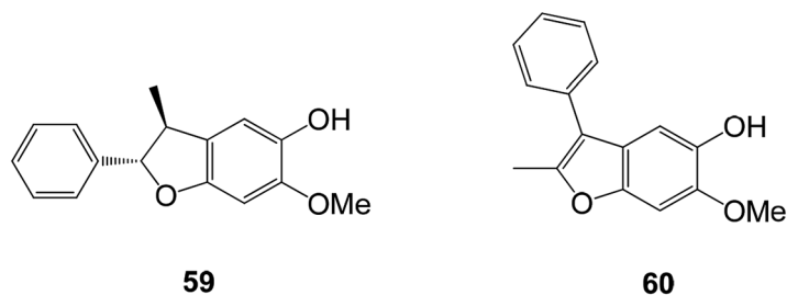
Fig. 22 Chemical structures of compounds 59 and 60.
