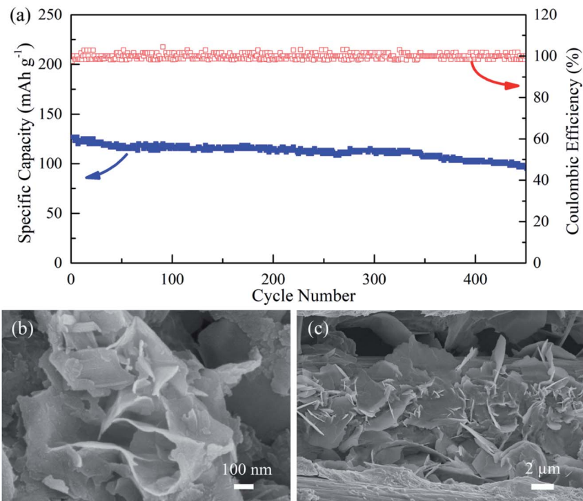
Fig. 3 (a) Cycling stability of the solid-state ZIBs with KCR electrolyte cycled at 6.0 \text{ A g}^{-1} and corresponding coulombic efficiency. SEM images of (b) the MnO 2 cathode and (c) the electroplated Zn anode after 450 charge/discharge cycles.
