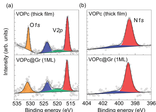
Fig. 2 XPS spectra of a VOPc thick film (top panels) and in the first monolayer on Gr/SiC(0001) (bottom panels): core-level spectra of O1s and V2p (a) and N1s (b). The region has been fitted using a linear background. (a) Red and blue components correspond to the V2p 3/2 and V2p 1/2 signals, a satellite peak is shown in green; the O1s region is fitted with a single component (orange). (b) N1s results in a main component (red) and a satellite peak (blue) at higher binding energy.
