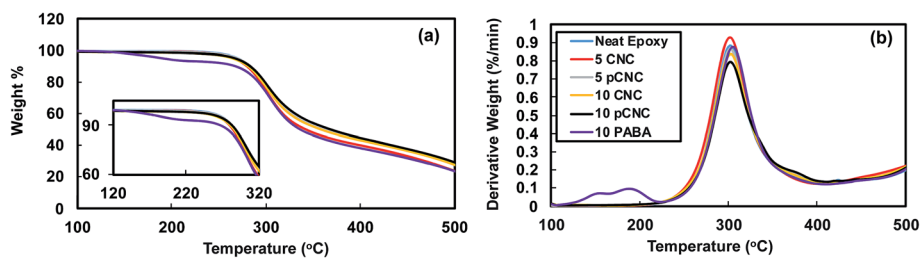
Fig. 10 TGA analysis of epoxy nanocomposites with different fillers. (a) Weight loss curve and (b) weight loss derivative curve.
