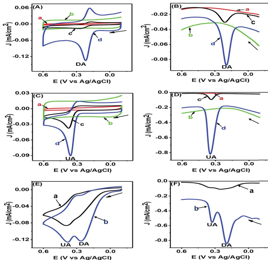
Fig. 7 (A) CVs and (B) DPVs of blank 0.1 M PBS solution of pH 7.0 (a and b) and 50 \mu M DA (c and d) in the same PBS of pH 7.0 at the GCE (a and c) and PTPCNs/GCE (b and d). CVs (C) and DPVs (D) of blank 0.1 M PBS of pH 7.0 (a and b) and 200 \mu M UA (c and d) in PBS of pH 7.0 at the GCE (a and c) and PTPCNs/GCE (b and d). CVs (E) and DPVs (F) of the mixture of 50 \mu M DA and 200 \mu M UA in 0.1 M PBS of pH 7.0 at the bare GCE (a) and PTPCNs/GCE (b).
