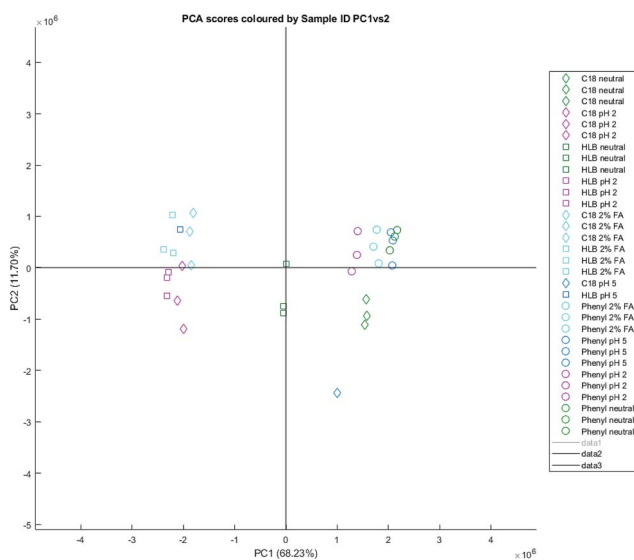
Fig. 3 A PCA scores plot based on reversed phase SPE elutions of natural urine, PC1 (68.23%) vs. PC2 (16.76%).
