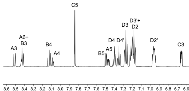
Fig. 6 Aromatic region of the ^1H NMR spectrum (500 MHz, acetone- d_6 ) of [Cu(Bu_2xantphos)(6-Mebpy)][PF_6] . See Scheme 3 for atom labelling.
