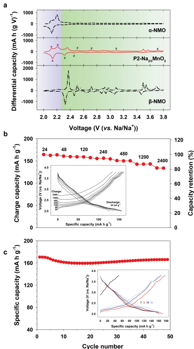
Fig. 4 Sodium storage performance of the nanostructured P2- \text{Na}_{2/3}\text{MnO}_2 . (a) Differential capacity plots at 12 \text{ mA g}^{-1} . Data for \alpha -NMO and \beta -NMO were adapted from ref. 32. (b) Rate performance at various charge current densities. (c) Cycling performance at 12 \text{ mA g}^{-1} (inset: corresponding voltage profiles).
