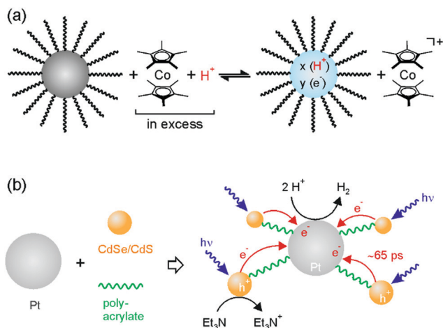
Fig. 8 (a) Chemical reduction of ZnO nanoparticles with CoCp 2 in presence of acid. 91 (b) the assembly of Pt nanoparticles with CdS/CdSe quantum dots via polyacrylate linkers leads to a system that is able to produce H 2 upon irradiation with visible light. 93
