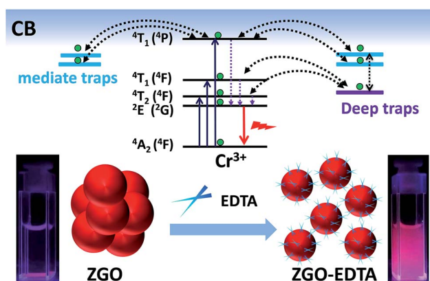
Scheme 1 The strategy of EDTA etching for regulating the traps, size and aqueous-dispersibility of ZGO.
