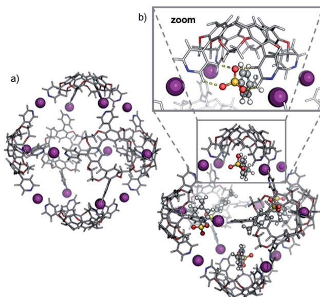
Fig. 4 Geometry-optimized structure of the hexameric halogen-bonded capsule 2 (a) in the absence of tosylate ions ( [\text{6} \cdot \text{C}_H + 12\text{I}]^{12+} ) and (b) with six tosylate anions ( [\text{6} \cdot \text{C}_H + 12\text{I} + 6 \cdot \text{OTs}]^{6+} ). The n -hexyl chains are omitted for clarity. Inset: binding situation of a tosylate counterion.
