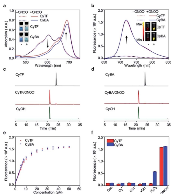
Fig. 1 UV-vis absorption spectra (a) and fluorescence spectra (b) of CyTF or CyBA (20 \mu\text{M} ) in the absence or presence of \text{ONOO}^- (25 \mu\text{M} ) at 25 ^{\circ}\text{C} in PBS (1x, pH = 7.4) containing 20% DMSO. Excitation: 640 nm. (c) High performance liquid chromatography (HPLC) traces of the incubation mixture of CyTF (c) and CyBA (d) in the absence (upper panel) or presence (middle panel) of \text{ONOO}^- (25 \mu\text{M} ), and HPLC traces of CyOH in water (lower panel). Wavelength: 600 nm. (e) Fluorescence titration of CyTF or CyBA (20 \mu\text{M} ) as a function of \text{ONOO}^- concentration. Each spectrum was recorded 5 min after addition of \text{ONOO}^- . Regression equation for CyTF : \text{FL} = 1.07 \times 10^6 + 1.16 \times 10^6 [\text{ONOO}^-] \mu\text{M} ( R^2 = 0.99 ); regression equation for CyBA : \text{FL} = 1.14 \times 10^6 + 1.27 \times 10^6 [\text{ONOO}^-] \mu\text{M} ( R^2 = 0.99 ). (f) Fluorescence intensity of CyTF and CyBA in the presence of various RONS for 5 min in PBS (1x, pH = 7.4) containing 20% DMSO. Control represents assay buffer only. \text{ONOO}^- was 25 \mu\text{M} , \text{O}_2^{\cdot-} , \text{OCl}^- , ^{\cdot}\text{OH} , and \text{H}_2\text{O}_2 were 50 \mu\text{M} . The incubation time for \text{H}_2\text{O}_2 was 2 hours. Error bars represent standard deviations of three separate measurements.
