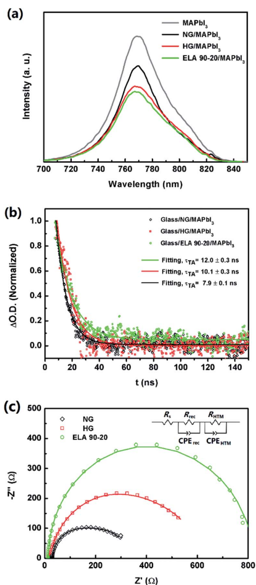
Fig. 7 (a) PL spectra of glass substrate/ETL/MAPbI 3 (ETL = NG, HG, ETL 90-20, or none) samples. (b) Transient absorption decay of glass substrate/ETL/MAPbI 3 (ETL = NG, HG, and ETL 90-20) samples. (c) Nyquist plots of the PHJ-PSCs based on NG, HG, and ELA 90-20. The inset is the equivalent circuit of the cell.
