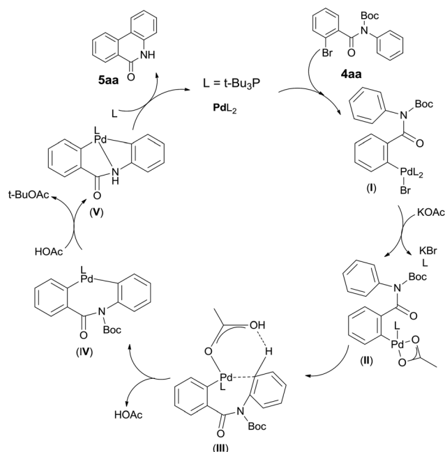
Scheme 3 Proposed mechanism for the phenanthridinone synthesis.
