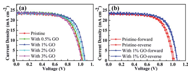
Fig. 1 (a) J – V curves of the fabricated champion PSCs with different amount of GO in the perovskite precursor solution; (b) the forward and reverse scans for the champion pristine PSC without GO and that with 1 vol% of GO.
