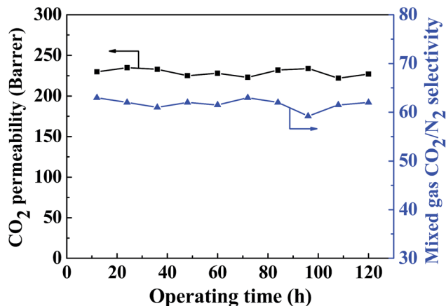
Fig. 14 Long-term operation stability of the gas separation performance observed for the MMM containing 20 wt% ZIF-8@GO.
