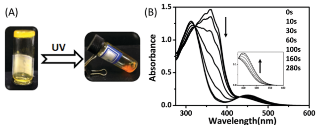
Fig. 5 (A) Photos showing gel-sol transition of trans -C 5 -Chol in DMF ( c = 62 mM) after 15 min of UV irradiation ( 90 mW \text{cm}^{-2} , 365 nm). (B) UV-Vis spectra of trans -C 5 -Chol in DMF solution ( c = 0.1 mM) with different UV irradiation time ( 0.25 mW \text{cm}^{-2} , 365 nm).
