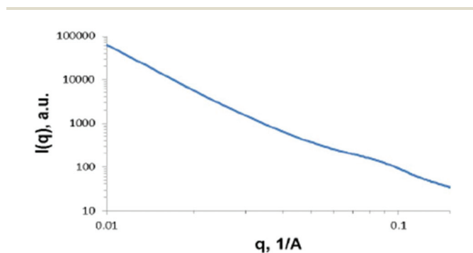
Fig. 4 Logarithmic plot of the scattering intensity ( I ) vs. scattering vector ( q ) for the C-MGultr sample.
