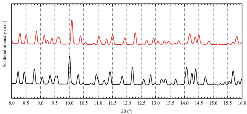
Fig. 10 X-ray diffraction patterns of the UiO-67-Pd sample taken during reduction in hydrogen at 33 °C (black) and 300 °C (red).
