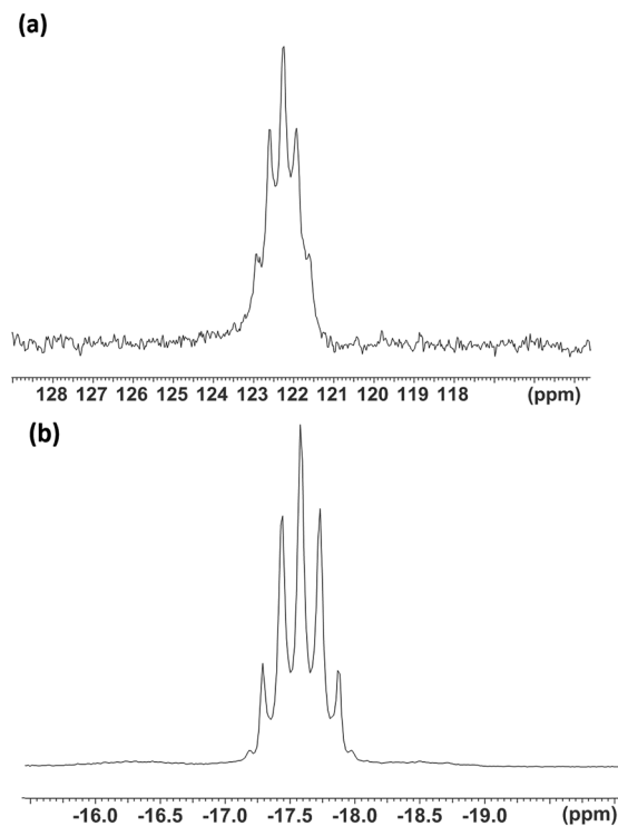
Fig. 3 The NMR spectra of [\text{WF}_4\{o\text{-C}_6\text{H}_4(\text{PMe}_2)_2\}_2]^{2+} : (a) ^{31}\text{P}\{^1\text{H}\} and (b) ^{19}\text{F}\{^1\text{H}\} in \text{MeCN} solution.
