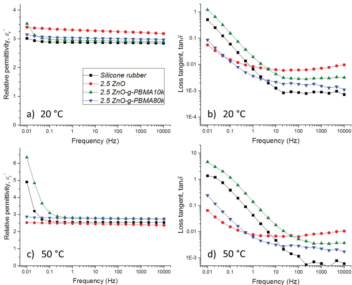
Fig. 12 Dielectric spectroscopy data of silicone rubber , 2.5\text{ZnO} , 2.5\text{ZnO-g-PBMA10k} and 2.5\text{ZnO-g-PBMA80k} at 20 °C (a and b), and 50 °C (c and d). Fig. (a) and (c) display the relative permittivity, \epsilon'_r versus frequency, and (b) and (d) the loss tangent, \tan \delta versus frequency.
