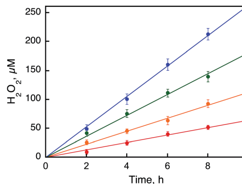
Fig. 4 Time courses of the photocatalytic production of \text{H}_2\text{O}_2 from \text{H}_2\text{O} and \text{O}_2 with [\text{Ru}^{\text{II}}(\text{Me}_2\text{phen})_3]^{2+} ( 0.10 \text{ mM} ) in the presence of a catalytic amount of 1 [ 0.50 \text{ mM} (red), 1.0 \text{ mM} (orange), 1.5 \text{ mM} (green), and 2.0 \text{ mM} (blue)] in an air-saturated solvent mixture of MeCN and \text{H}_2\text{O} ( v/v = 23 : 2 ) containing \text{Sc}(\text{NO}_3)_3 ( 100 \text{ mM} ) under photoirradiation (white light) at 298 \text{ K} .
