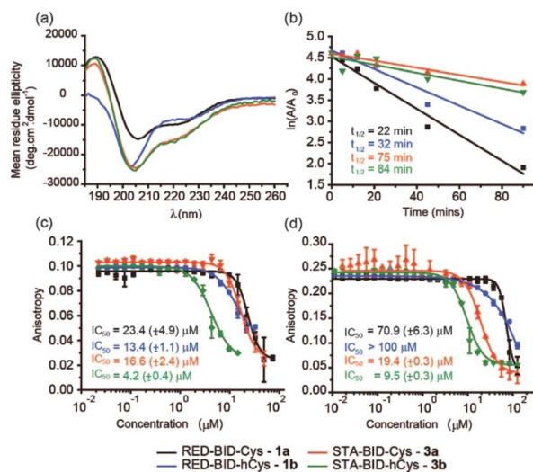
Fig. 3 Analyses on BID derived peptides 1a,b and 3a,b . (a) Circular dichroism spectra (water/30% acetonitrile); (b) trypsin proteolysis in a 1 : 10 000 enzyme/substrate ratio (50 mM phosphate buffer, 200 mM NaCl, pH 7.50); (c) fluorescence anisotropy competition assay for inhibition of the FITC-BID/Mcl-1 interaction (25 nM tracer, 150 nM protein, 50 mM Tris buffer, 150 mM NaCl, 0.61% of Triton X-100, pH 7.40); (d) fluorescence anisotropy competition assay for inhibition of the BODIPY-BAK/Bcl-x L interaction (25 nM tracer, 150 nM protein, 50 mM phosphate buffer, 200 mM NaCl, 0.02 mg mL -1 BSA, pH 7.50).
