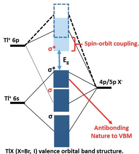
Fig. 1 Schematic representation of the valence orbital band structure of \text{TlX} ( X = \text{Br} and \text{I} ) showing the bonding and antibonding orbitals forming the energy bands of the \text{TlX} solid, relative to the isolated p and s atomic orbitals of \text{Tl}^+ and \text{X}^- , respectively. The non-bonding \text{Tl} 6p states mainly constitute the conduction band minimum (light-blue band), which is further stabilized by strong spin-orbit coupling. The anti-bonding interactions of \text{Tl} 6s and \text{X} np constitute the valence band (dark-blue) maximum.
