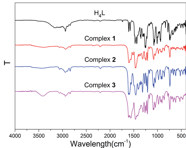
Fig. 1 IR spectra of the ligand H_4L and its corresponding complexes 1–3.
