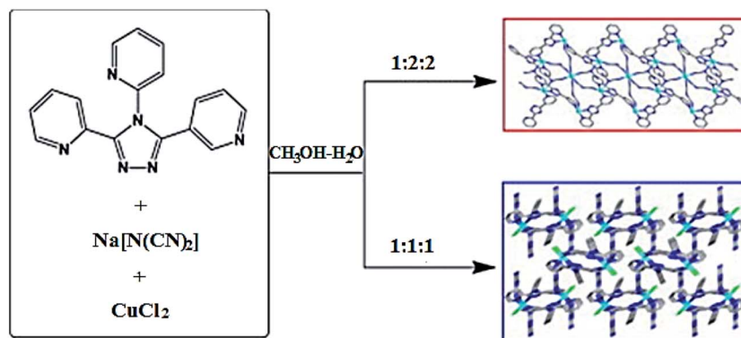
Scheme 11 The assemblies of the tripyridyltriazole ligand 3,4-bis(2-pyridyl)-5-(3-pyridyl)1,2,4-triazole with \text{Cu}(\text{II}) chloride and dca anion at different \text{M-L} ratios into CPs displaying 1D double-chained massif and 3D chiral dia network, respectively. [Reprinted from ref. 137. Copyright 2014, with permission from Elsevier.]
