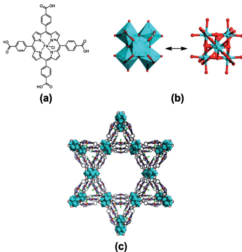
Fig. 2 (a) \text{FeL}^1 -Cl metalloligand. (b) \text{Zr}_6\text{O}_8(\text{CO}_2)_8(\text{H}_2\text{O})_8 SBU. (c) Hexagonal and triangular 1D channels of MMPF-6. Color scheme: C, gray; O, red; Cl, green; Zr, turquoise. [Reprinted with permission from ref. 57. Copyright 2012, American Chemical Society.]
