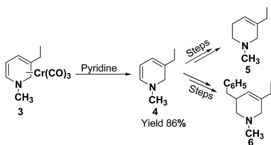
Scheme 2 Dihydropyridine 4 generated from precursor chromium complex 3.
