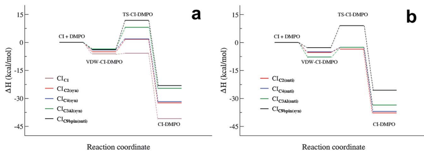
Fig. 4 Reaction energy profiles of the CI + DMPO \rightarrow CI-DMPO reactions of C1C1, C1C2, C1C4, C9pin and C1C3Al, calculated starting from the more stable (a) and the less stable (b) conformation of each adduct.
