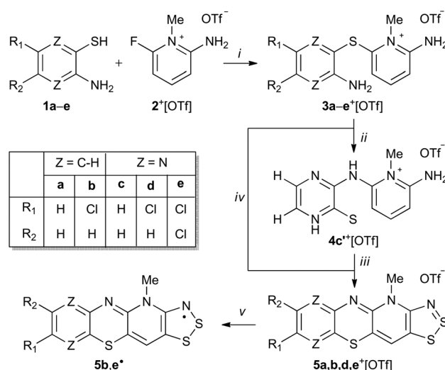
Scheme 1 Synthesis of neutral radicals 5 • . Reagents and general conditions: (i) Na 2 CO 3 , MeCN, 5 h; (ii) MeCN, sealed vessel, 110 °C; (iii) excess S 2 Cl 2 , MeCN, reflux, 16 h; (iv) excess Me 8 Fc, MeCN. Highest yields obtained: 4c •+ [OTf] 79%, 5a •+ [OTf] 2%, 5b •+ [OTf] 43%, 5d •+ [OTf] 48%, 5e •+ [OTf] 78%, 5b • 81%, and 5e • 70%.
