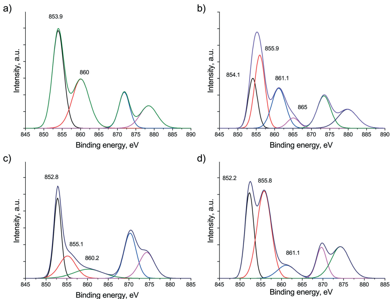
Fig. 2 Ni 2p region measured by XPS after calcination at 600 °C on (a) \text{Ni/ZrO}_2 and (b) \text{Na-Ni/ZrO}_2 and after reduction at 600 °C on (c) \text{Ni/ZrO}_2 and (d) \text{Na-Ni/ZrO}_2 . Fitted curves are shown.
