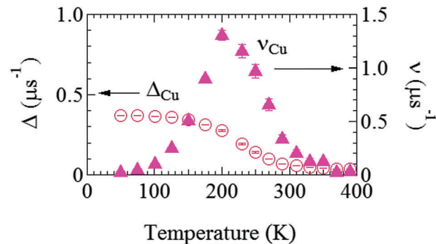
Fig. 6 The temperature dependences of field distribution width ( \Delta_{Cu} ) (left) and field fluctuation rate ( \nu_{Cu} ) (right) of the Cu foil. The data were obtained by fitting the \mu^+ SR spectra for the Cu foil with eqn (1) but A_{C_6Li} = 0 .
