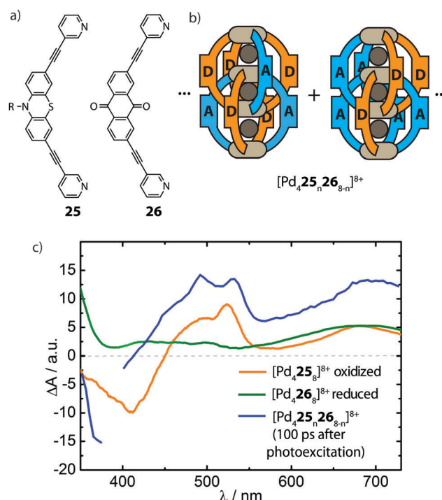
Fig. 15 (a) Electron-donor (25) and acceptor (26) ligands; (b) representation of the statistical composition of the mixed-ligand double-cages; (c) time-resolved pump-probe UV-Vis spectrum of photo-excited mixed-ligand cages compared to the spectra of the oxidized donor and reduced acceptor cages, respectively.
