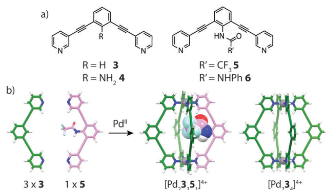
Fig. 5 (a) Endohedrally functionalized ligands 3–6 bearing varying degrees of steric bulk; (b) integrative self-sorting of ligands 3 and 5 to give a 3 : 1 mixture of [Pd 2 3 3 5] 4+ and [Pd 2 3 4 4] 4+ . The NHCOCF 3 endohedral substituent in the heteroleptic assembly is shown as a space-filling representation.
