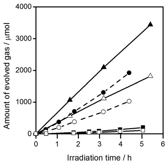
Fig. 5 Gas evolution during the water splitting reaction on Al-STO(-flux-Y). H 2 (■) and O 2 (□) on 0.1%Al-STO(flux-Y), H 2 (●) and O 2 (○) on 1%Al-STO(flux-Y), and H 2 (▲) and O 2 (△) on 10%Al-STO(flux-Y). Reaction conditions: catalyst, 0.1 g; cocatalyst, Rh 2-y Cr y O 3 (Rh 0.1 wt%, Cr 0.1 wt%); reaction solution, 100 mL H 2 O; light source, 300 W Xe lamp ( \lambda > 300 nm).
