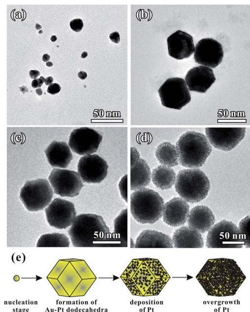
Fig. 3 TEM images of the typical porous rhombic dodecahedral AuPt@Pt bimetallic NCs obtained using the standard procedure at different reaction times, (a) 1 min, (b) 5 min, (c) 10 min and (d) 1 h, showing the evolution of morphology with time. (e) A schematic illustration showing the formation process of the Au–Pt bimetallic NCs.
