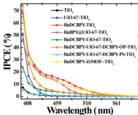
Fig. 2 Incident photon to current conversion efficiency (IPCE) spectra of unmodified TiO 2 (black), RuDCBPY on TiO 2 (red), undoped UiO-67–TiO 2 (blue), RuBPY@UiO-67–TiO 2 (pink), RuDCBPY–UiO-67–TiO 2 (green), RuDCBPY–UiO-67–DCBPY-OP–TiO 2 (orange), RuDCBPY–UiO-67–DCBPY-PS–TiO 2 (cyan), and RuDCBPY–ZrMOF–TiO 2 (yellow) collected in a tetrabutylammonium iodide (TBAI) and iodine based electrolyte in CH 3 CN with a platinum counter electrode.
