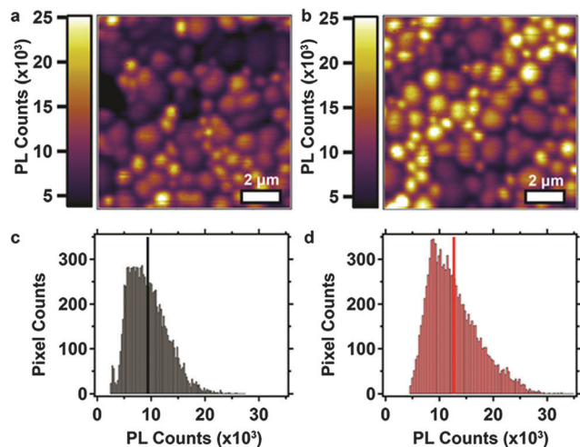
Fig. 4 Fluorescence microscopy of (a) control and (b) \text{Al}^{3+} -doped (0.15 mol%) perovskite films with 10 \times 10 \mu\text{m} area mapping excited with a pulsed 470 nm laser (40 MHz, 117 ps pulse width, 300 \text{ nJ cm}^{-2} per pulse). (c and d) Are the image histograms (10 000 pixels) showing the fluorescence emission distribution with solid lines indicate the average number of PL counts. The \text{Al}^{3+} -doped perovskite has more pixel counts falling under "bright" regions as compared to the control.
