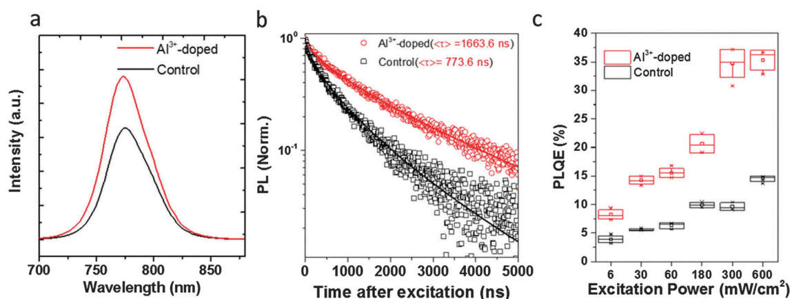
Fig. 3 Photoluminescence spectroscopy of control (non-doped) and 0.15 mol% \text{Al}^{3+} -doped perovskite thin films deposited on glass substrate with (a) steady-state spectra ( 300 \text{ mW cm}^{-2} , 507 \text{ nm} ), (b) time-resolved photoluminescence decay after excitation at 507 \text{ nm} with pulsed ( 200 \text{ kHz} ) and a fluence of 30 \text{ nJ cm}^{-2} per pulse, and (c) photoluminescence quantum efficiency (PLQE) as a function of excitation power (further details are available in the ESI † ).
