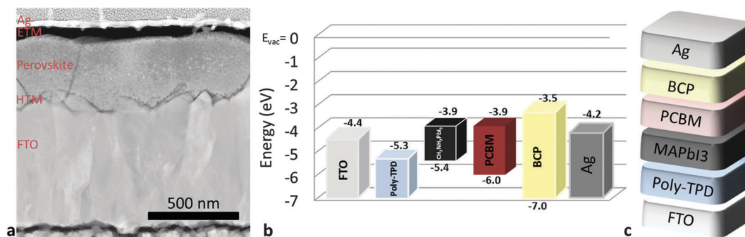
Fig. 5 (a) High angle annular dark field STEM (HAADF-STEM) cross-sectional micrograph of optimized device with the structure of Ag/BCP/ETM (PCBM)/perovskite/HTM (poly-TPD)/FTO. (b) Diagram of the energy levels of the materials used and (c) an illustration of the structure of the solar cells.
