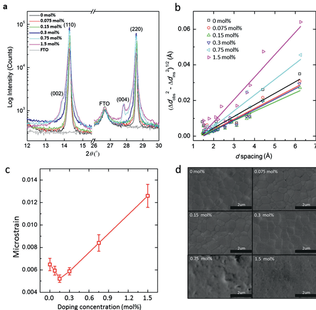
Fig. 1 Characterizations of control and \text{Al}^{3+} -doped perovskite samples with (a) X-ray diffraction patterns analysis, and (b) a modified Williamson–Hall plot of (\Delta d_{\text{obs}}^2 - \Delta d_{\text{ins}}^2)^{1/2} versus d spacing extracted from the corresponding diffraction profiles shown in Fig. S1 (ESI†). The slopes of the solid lines from linear fits indicate the extents of microstrain at different doping concentrations. (c) Calculated microstrain of samples with different \text{Al}^{3+} doping concentration from XRD patterns (the error bars for each concentration in the plot c, are determined from the fits in b). (d) Top view scanning electron microscope (SEM).
