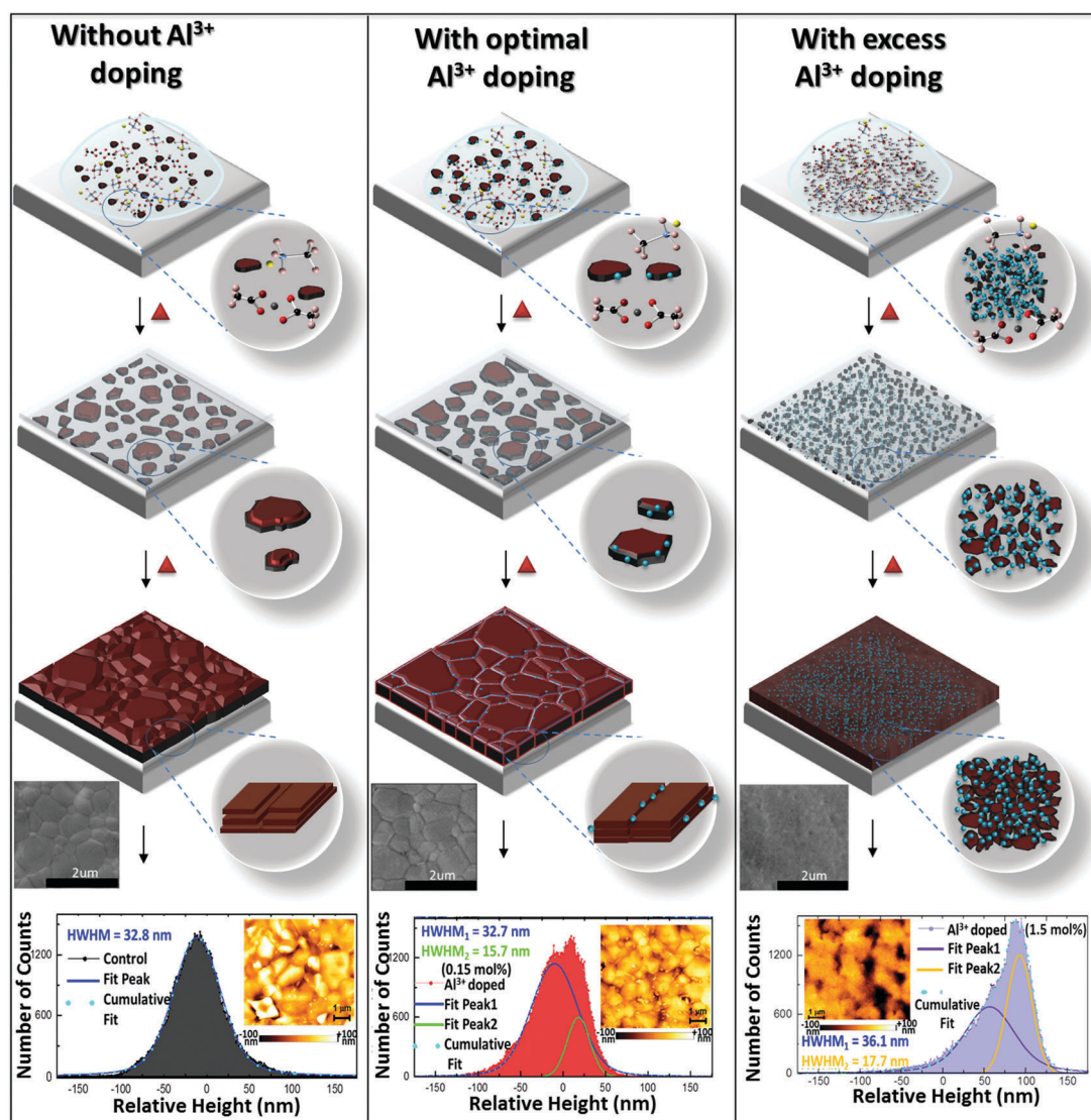
Fig. 2 Schematic diagram of the proposed perovskite polycrystalline thin film growth and influence of the \text{Al}^{3+} doping with illustrated C, N, H, O, I, Pb, and Al atoms are indicated by the color of black, blue, pink, red, grey, and cyan respectively; and histograms of the surface topography and the images (insets) from AFM measurements of different samples. Best fits for the histograms are obtained using one and two Voigt distributions, respectively for the control and the optimized sample. The individual distribution components with their HWHM, and the cumulative fits are labelled as in the figure.
