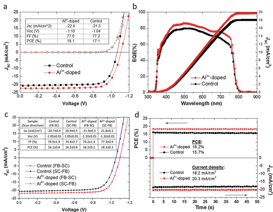
Fig. 6 Photovoltaic performance of control and \text{Al}^{3+} -doped (0.15 mol%) perovskite solar cells under simulated AM 1.5, 100 \text{ mW cm}^{-2} solar irradiation (solid line), and in the dark (dotted line) at a scan rate of 0.38 \text{ V s}^{-1} . (a) The current density–voltage characteristics of the best cells. (b) External quantum efficiency (EQE) spectrum measured at short-circuit, along with the expected photocurrent integrated over the AM 1.5 solar spectrums of 100 \text{ mW cm}^{-2} . (c) Numerically averaged JV curves measured from forward bias (FB) to short-circuit (SC) and back again without observable hysteresis in a selection of 20 high performance control and \text{Al}^{3+} doped devices. (d) Stabilized maximum power output measurement of the best cells with bias at their maximum power points.
