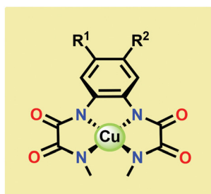
Fig. 54 Cu(II) complexes 161–164 based on tetradentate amidate ligands.
