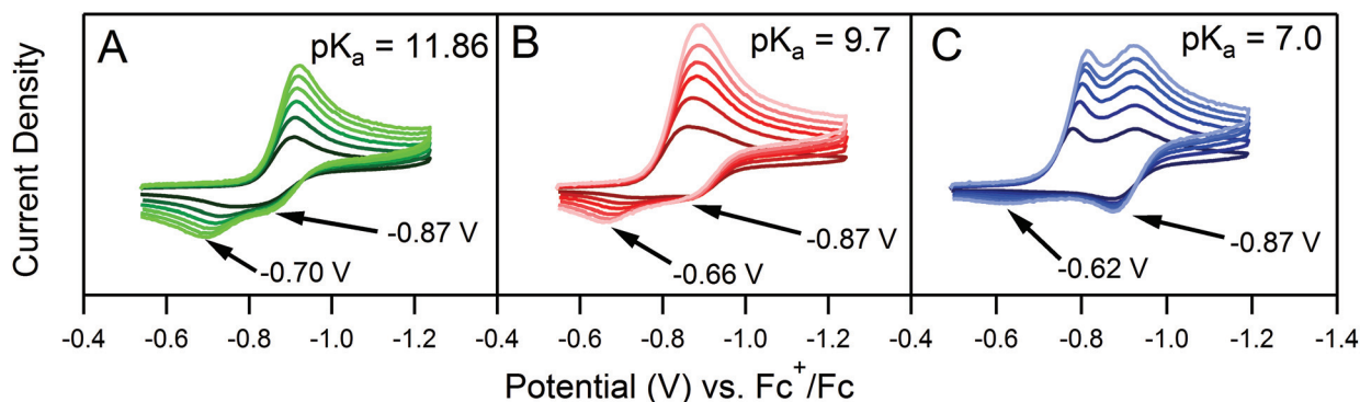
Fig. 2 Three sets of cyclic voltammograms recorded from solutions containing 0.5 mM \mathbf{1} and 0.5 mM (A) 4-methoxyanilinium, (B) 4-chloroanilinium, (C) 4-cyanoanilinium. Each set of data consists of six voltammograms recorded at 100, 200, 300, 400, 500, and 600 \text{mV s}^{-1} . All voltammograms recorded in a 250 mM [\text{Bu}_4\text{N}][\text{PF}_6] \text{CH}_3\text{CN} solution.
