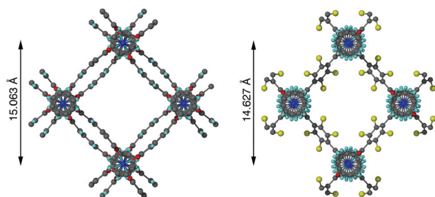
Fig. 1 Pore structure of [\text{Zn}_2(\text{bdc})_2(\text{dabco})]\cdot 4\text{DMF}\cdot 0.5\text{H}_2\text{O} (left) and [\text{Zn}_2(\text{bdc-Br})_2(\text{dabco})]\cdot n\text{DMF} (right), the latter showing a slight diagonal compression of the pore with the addition of bromine substituents into the framework. The bromine atom in [\text{Zn}_2(\text{bdc-Br})_2(\text{dabco})] is disordered over four positions.
