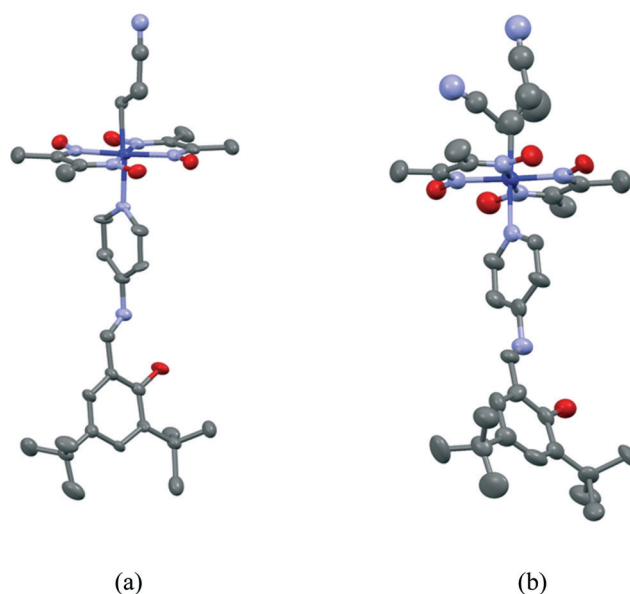
Fig. 10 Molecular structures of II before (a) and after (b) visible-light irradiation. Hydrogen atoms are omitted for clarity. The minor parts of the disordered salicylideneaniline moiety and 2-cyanoethyl group in (a) and the salicylideneaniline moiety in (b) are omitted for clarity.
