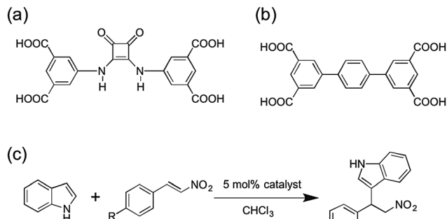
Fig. 1 (a) Structure of the H_4dbda ligand. (b) Structure of H_4tptc ligand. (c) Friedel–Crafts reaction between indole and substituted \beta -nitrostyrenes.
