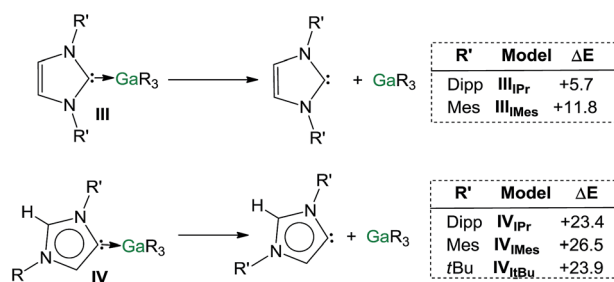
Fig. 7 Estimated dissociation energies ( \text{kcal mol}^{-1} ) of complexes III and IV ( \text{R} = \text{Dipp, Mes, } ^t\text{Bu} ).
