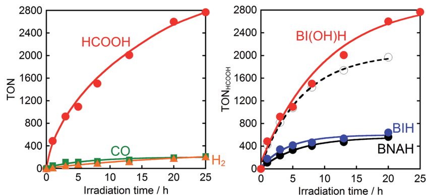
Fig. 2 (a) Photocatalytic formation of formic acid (●), CO (■), and H 2 (▲) as a function of irradiation time. (b) Photocatalytic formation of formic acid using BI(OH)H (●), BIH (●) or BNAH (●) as a sacrificial electron donor: a CO 2 saturated DMF-TEOA (4 : 1 v/v, 2 mL) solution containing Ru 2 -Ru(CO) (0.025 mM) and a sacrificial electron donor (0.1 M) was irradiated using \lambda_{\text{ex}} > 500 nm light (LIC2). Open circles (c) show the results obtained from the photocatalysis using BI(OH)H (0.1 M) and a mixed system of [Ru(dmb) 3 ] 2+ (0.05 mM) and cis -[Ru(dmb) 2 (CO) 2 ] 2+ (0.025 mM) instead of Ru 2 -Ru(CO).
