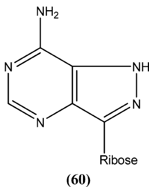
Formycin A
