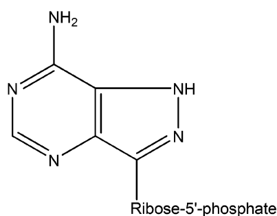
(62)
